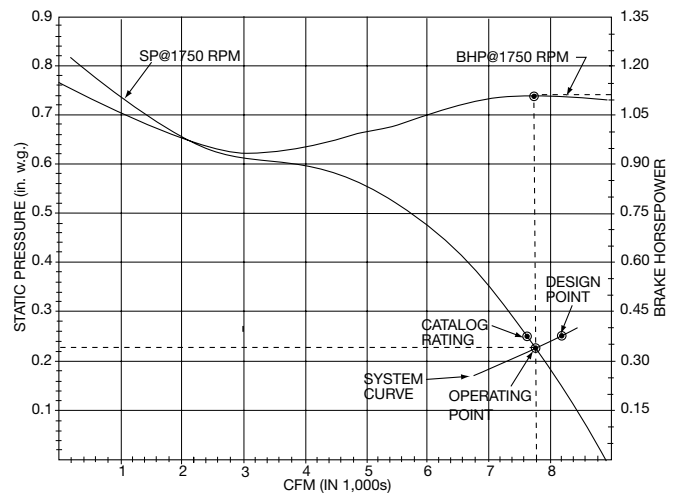
Figure 1. 24L230 Performance Curve
