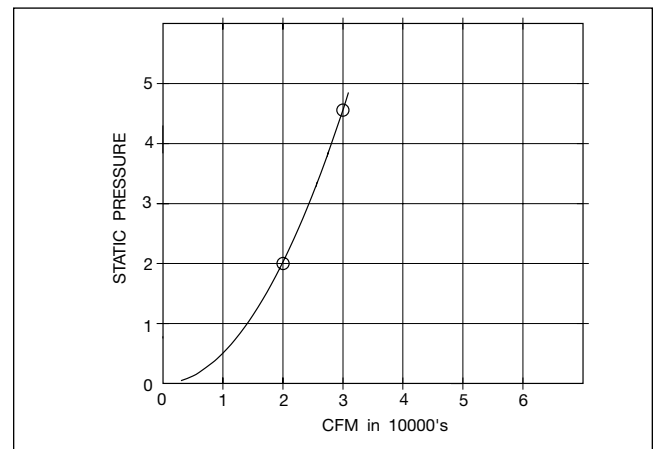
Figure 4. Two Performance Points Along the System Curve
