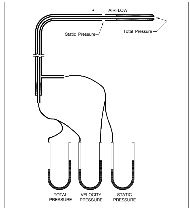
Figure 1. Pitot Tube
