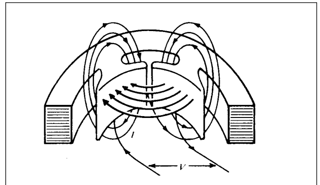
Figure 5. Flux Patterns Produced in Stator
