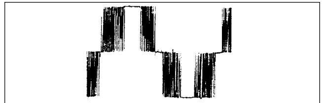
Figure 5. Pulse width modulated sine wave (line voltage from inverter)
