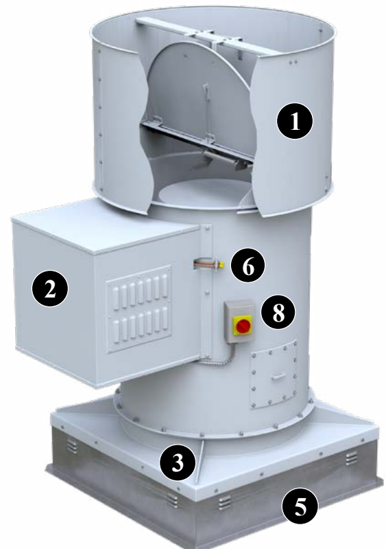
Model AMXSH (Smoke & Heat Fan)
