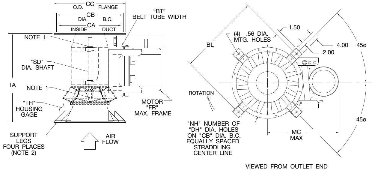
TYPE "AMX" VERTICAL UP DISCHARGE WITH FLOOR MOUNT SUPPORT LEGS
