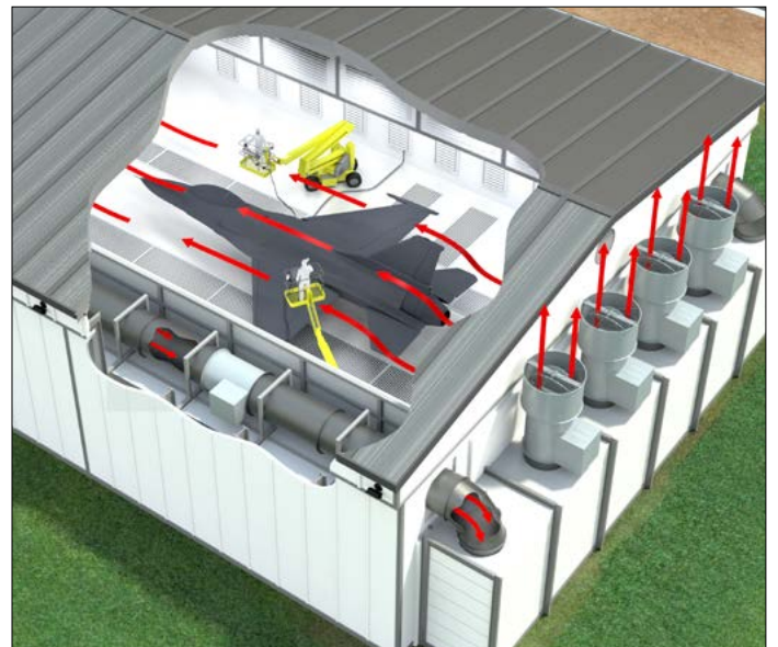
Paintbooth Application (Model AMX)
