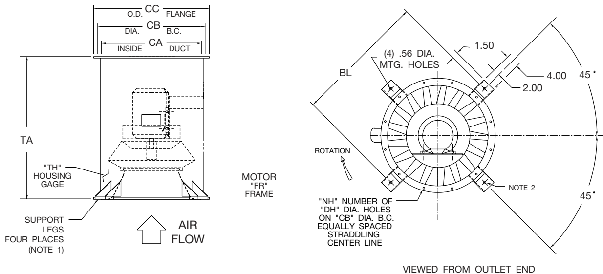
TYPE "AMX" VERTICAL UP DISCHARGE WITH FLOOR MOUNT SUPPORT LEGS (NOTE 1)
