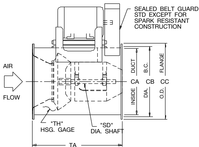
TYPE "AMX" HORIZONTAL DISCHARGE
