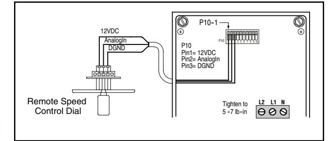
Figure 6. Motor Speed Controlled by a Remote Speed Control Dial (Potentiometer)
