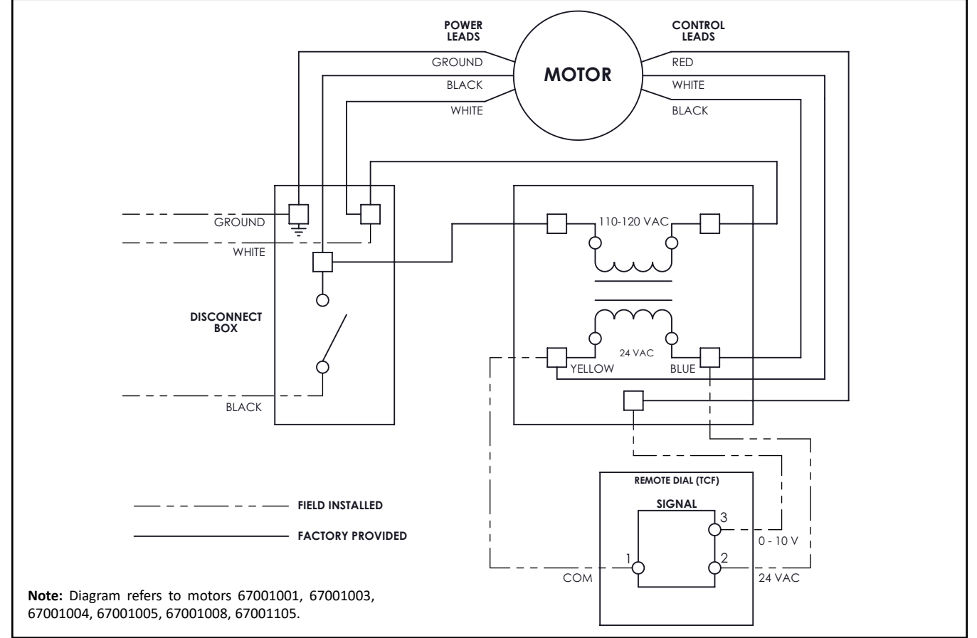
Figure 1. Remote Mounted Dial Wiring Diagram — 115VAC Single-Phase
