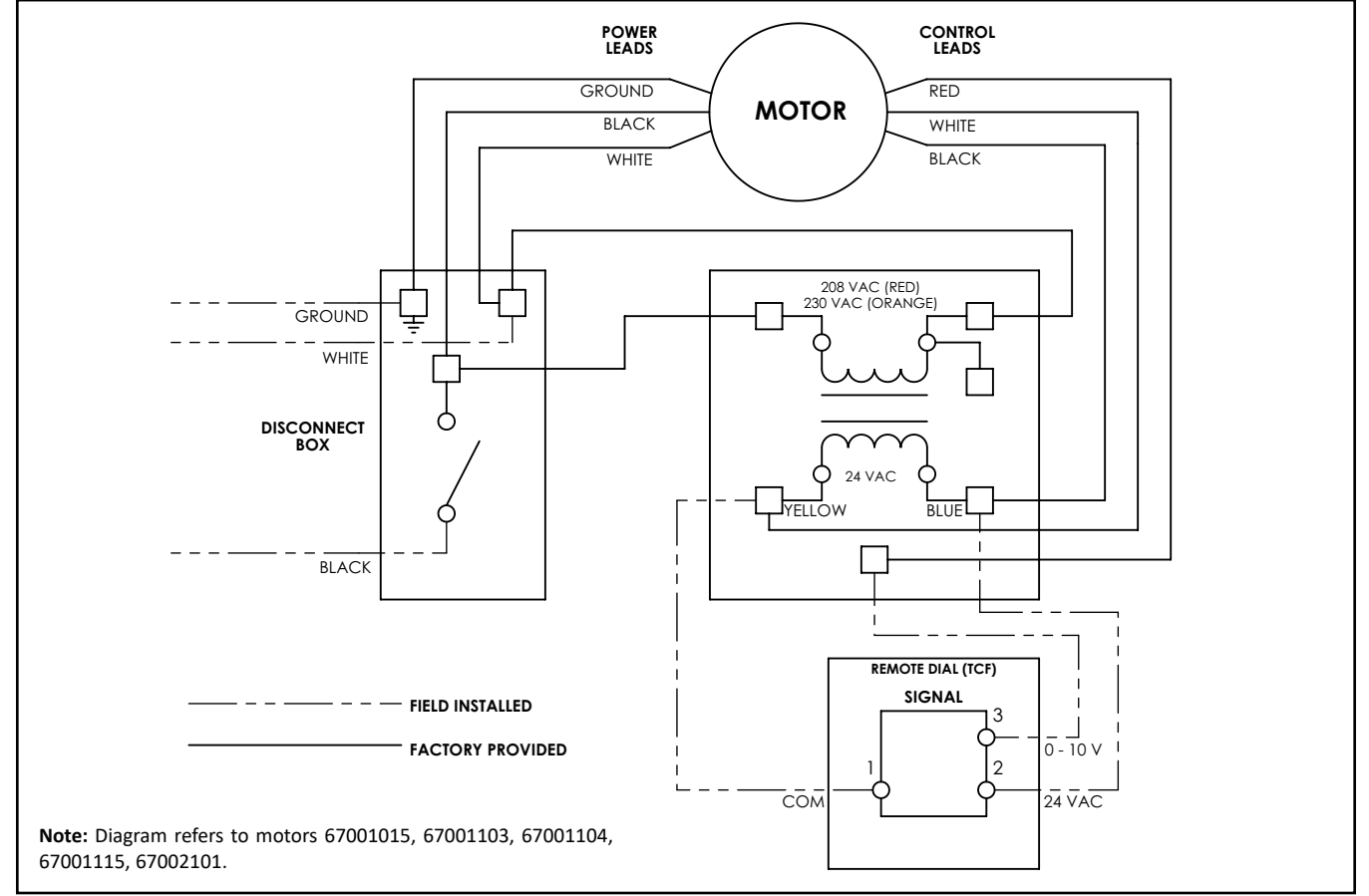
Figure 2. Remote Mounted Dial Wiring Diagram — 208-230VAC Single-Phase
