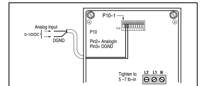
Figure 7. Motor Speed Controlled by 0-10V DC Control Signal
