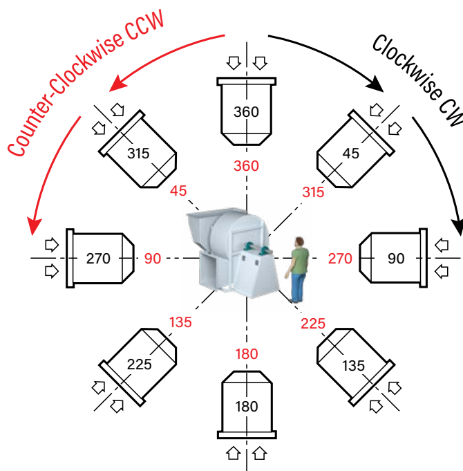
Inlet box positions determined from Drive Side.
